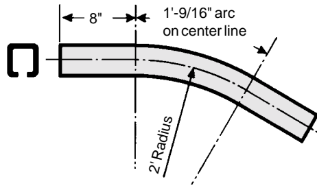
2'-0" RAD. 30° Upper Vertical Curve V20111
