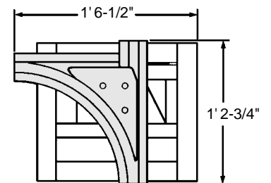
Universal Switch LH-V65528 (shown) RH-V65529
