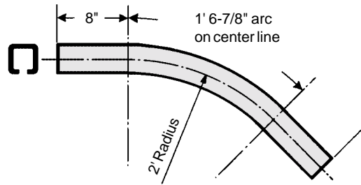
2'-0" RAD. 45° Upper Vertical Curve V20113
