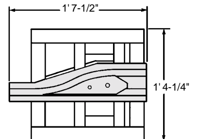
Universal Switch LH-V65528 (shown) RH-V65529
