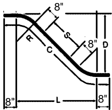
2'-0" RAD. 45° Upper Vertical Curve V20113
