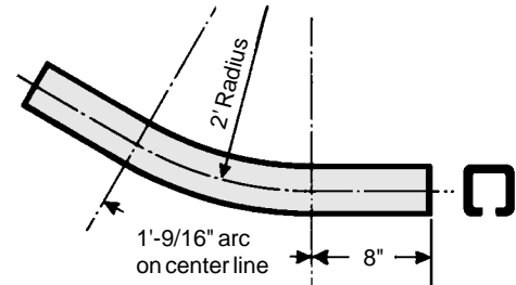
2'-0" RAD. 30° Upper Vertical Curve V20111
