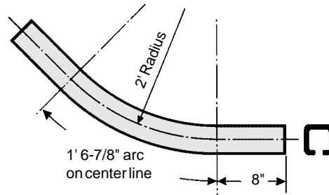
2'-0" RAD. 45° Upper Vertical Curve V20113
